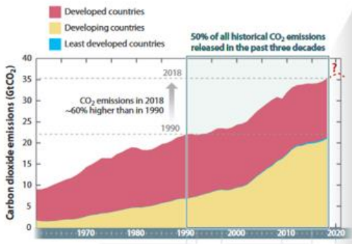
a Global carbon dioxide emissions*
